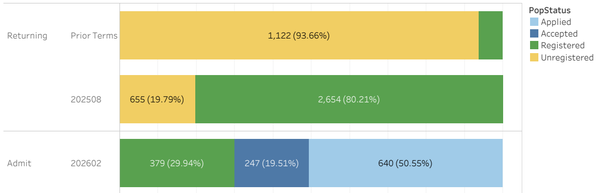
Student Group Population Status
